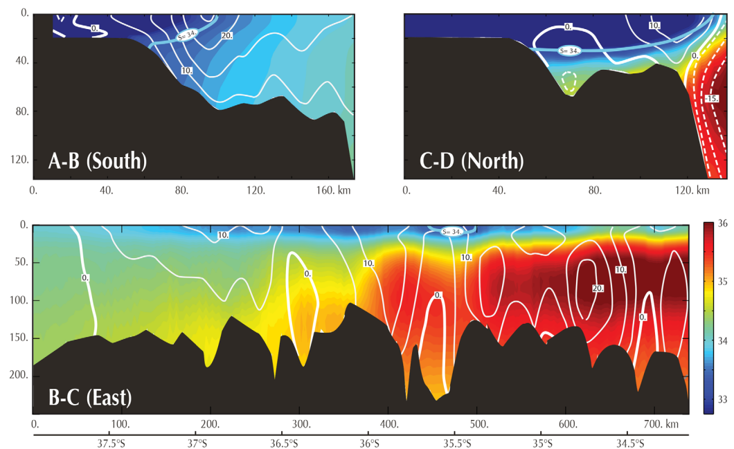
Figure 15. Mean vertical structure of the cross sections shown in Figure 14. The background colors represent the salinity field and the white contours are for the velocities (cm/s). The light-blue contours mark the 34 isohaline, which represents the limit of the LPR waters.
