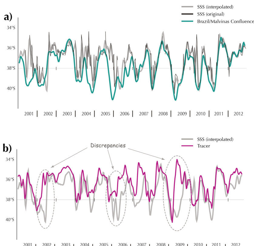
Figure 4. (a) Time series of the escape latitude calculated using the SSS criterion (Elis). The thin, black line represents the original time series, the thick gray line the interpolated value and the green line the time series of the latitudinal variations of the BMC. (b) Time series of the escape latitude calculated using the passive tracer (ELT, purple line) and using the SSS criterion (ELs, gray line).
